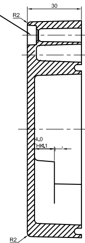
SECTION -B-B
