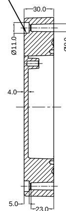
SECTION B-B
